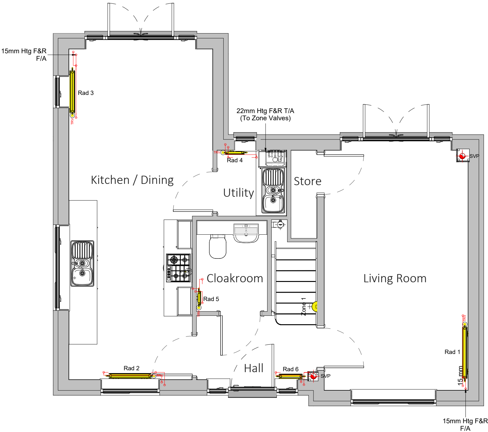
1 Ground Floor Heating GA 1 : 50
